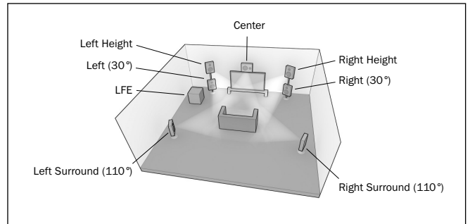
Configuration 5 - 7.1 channel: L, C, R, LFE, Ls, Rs, Lsr, Rsr
